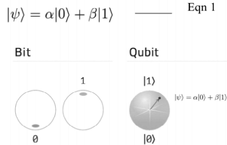
Figure 2: A comparison of states in a bit and Qubit
