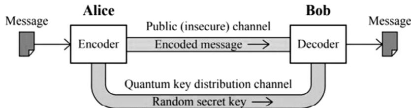
Figure 6: Quantum Cryptography [14]
