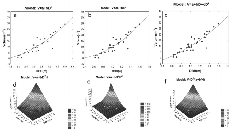
Figure.2 (a-f). Scatter plot of diameter at breast height versus volume ofthe Pinus roxburghii trees in Pithoragarh District.
